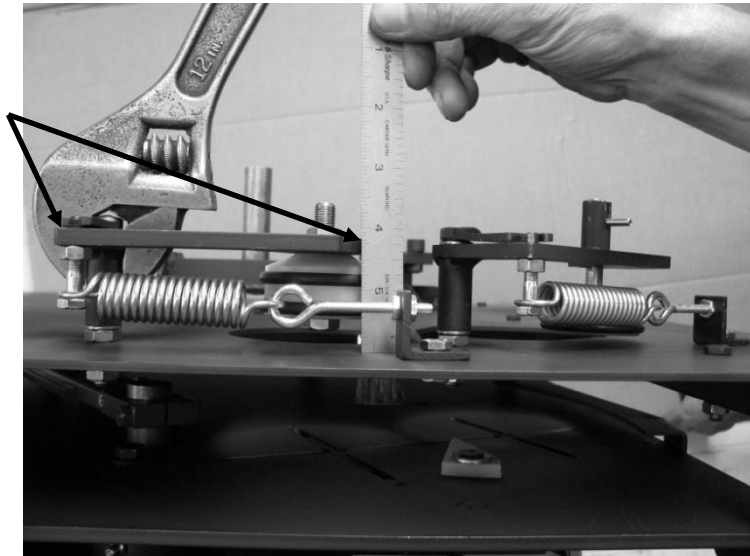
Adjusting height of Single Roller Plate
