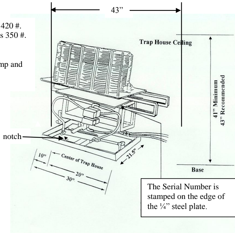
Base Dimensions of PAT-TRAP ®
